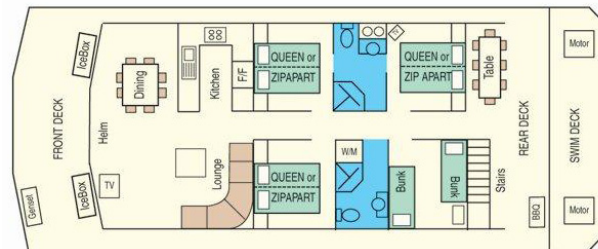
Floor Plan 18.6m x 8m
